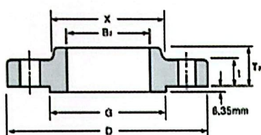
Slip-on
