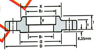
Socket Welding
